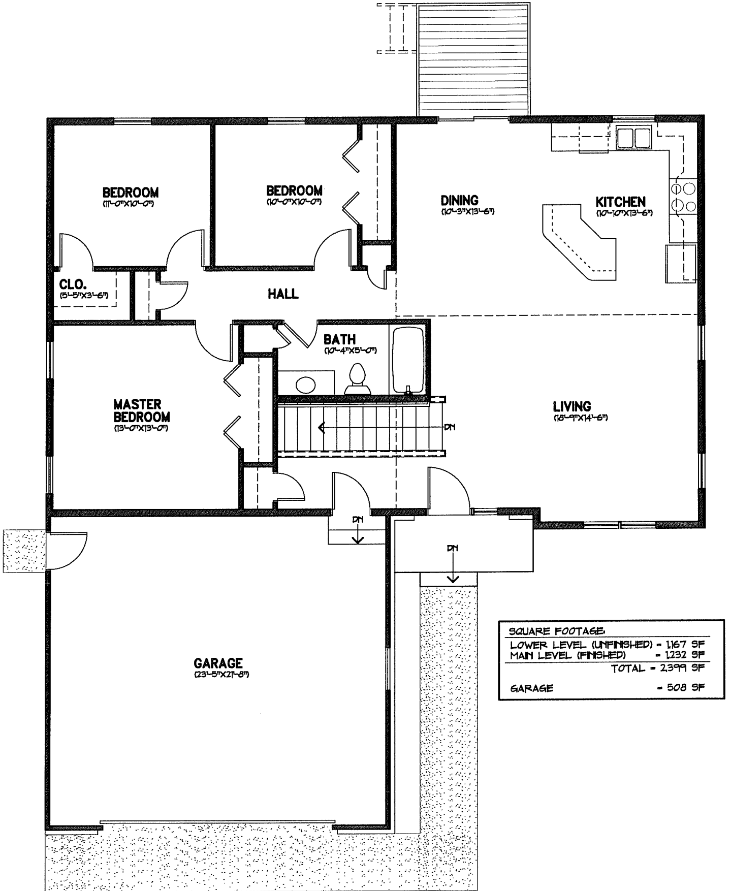
MAIN LEVEL PLAN
